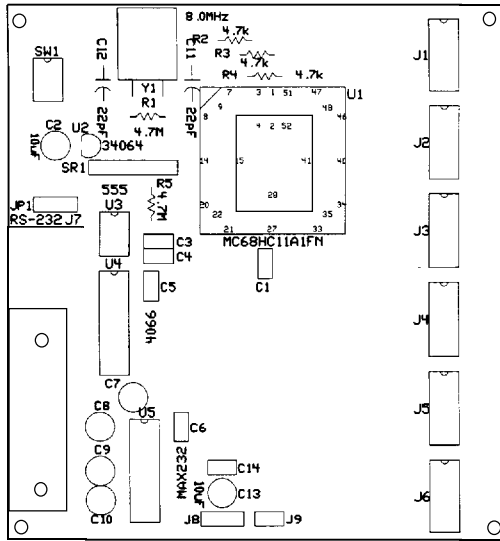
Figure 1. SBC-2A PC Board Layout
